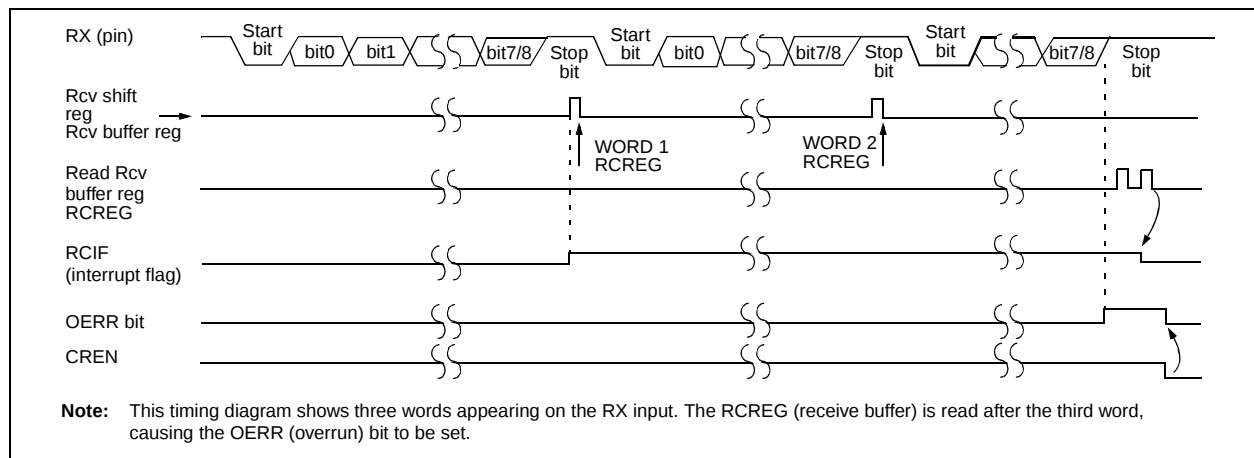
FIGURE 10-5: ASYNCHRONOUS RECEPTION
