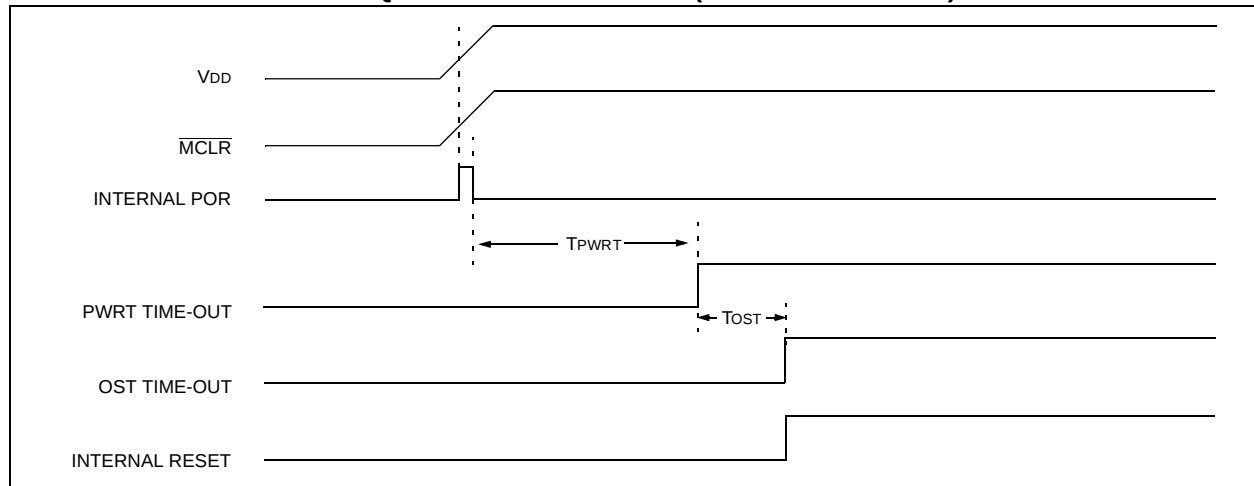
FIGURE 12-5: TIME-OUT SEQUENCE ON POWER-UP ( \overline{\text{MCLR}} TIED TO \text{V}_{\text{DD}} )
