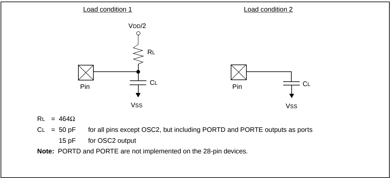
FIGURE 15-4: LOAD CONDITIONS
